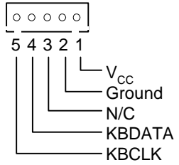
CN1 : AT Keyboard
