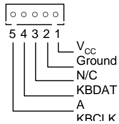
CN6 : AT Keyboard
