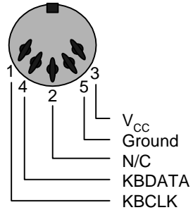
KB1 : AT Keyboard
